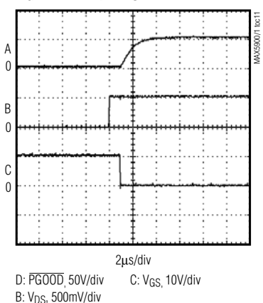
CIRCUIT-BREAKER EVENT ( C_{GATE} = 1000pF , V_{OVERDRIVE} = 200mV )
